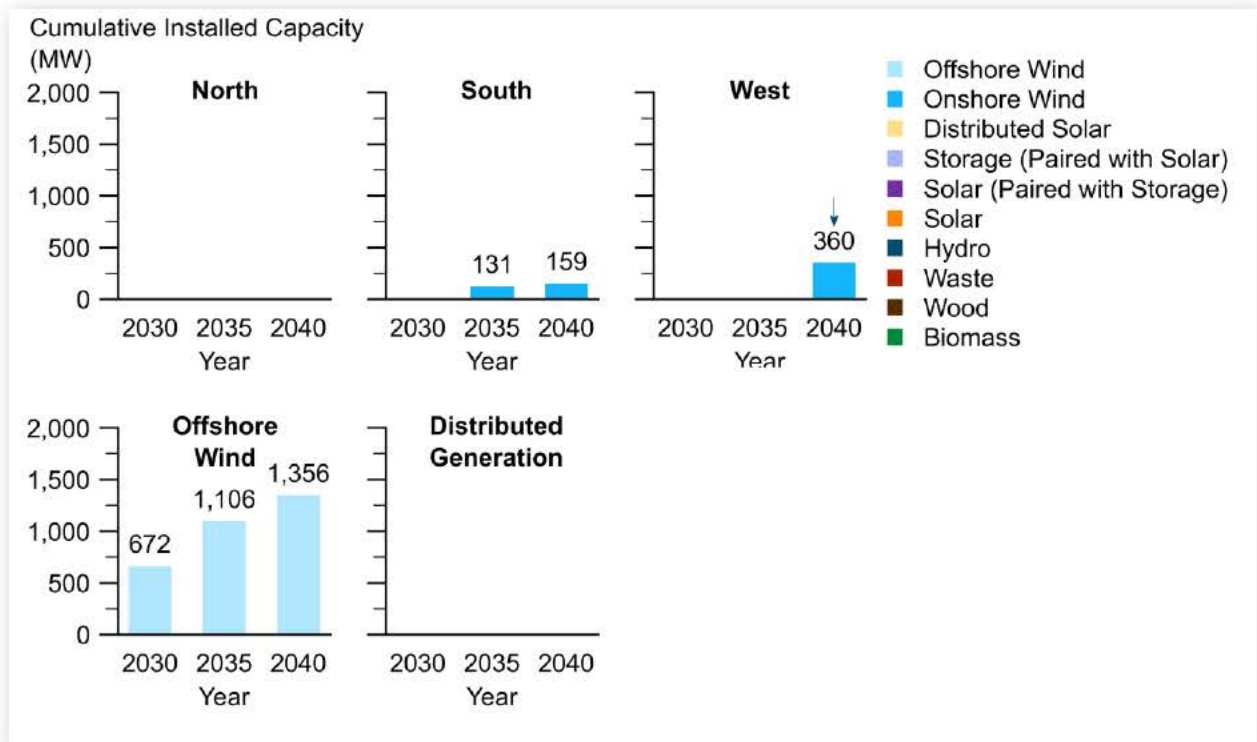
Figure 35. Regional build for the High Offshore Wind scenario. The year where the first or second transmission upgrades are needed in each region is indicated by a blue or red arrow, respectively.
