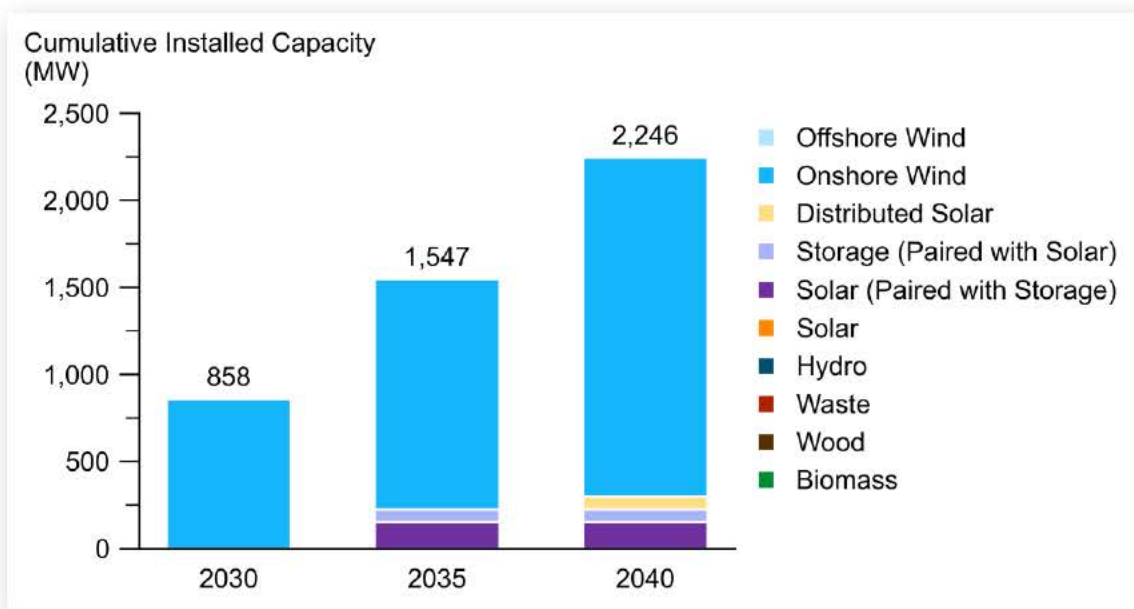
Figure 27. Renewable build in Maine in Base Case.
