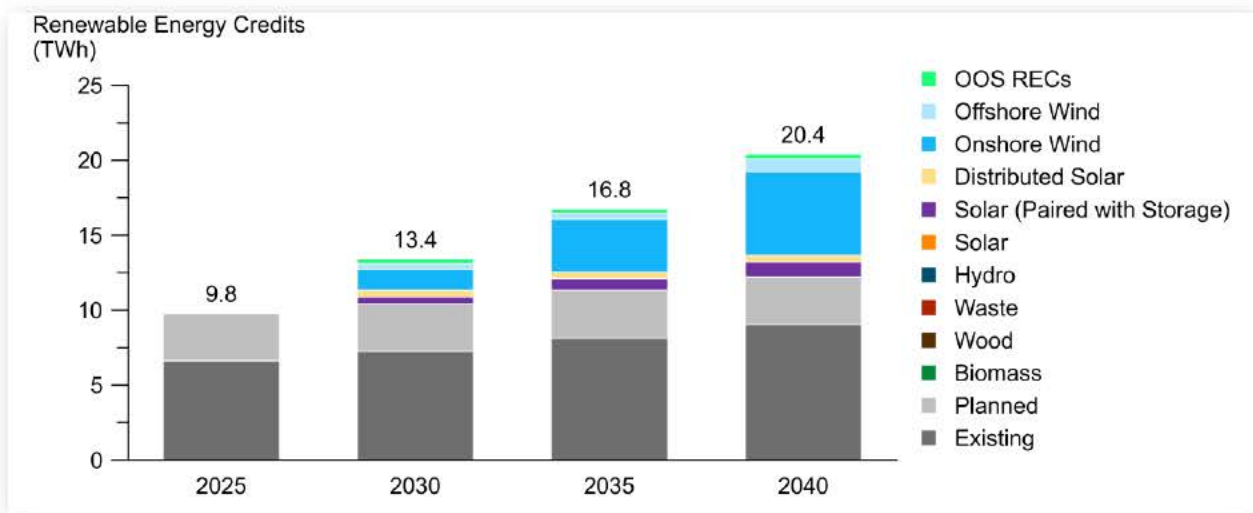
Figure 45. RECs for Diverse Portfolio scenario.
