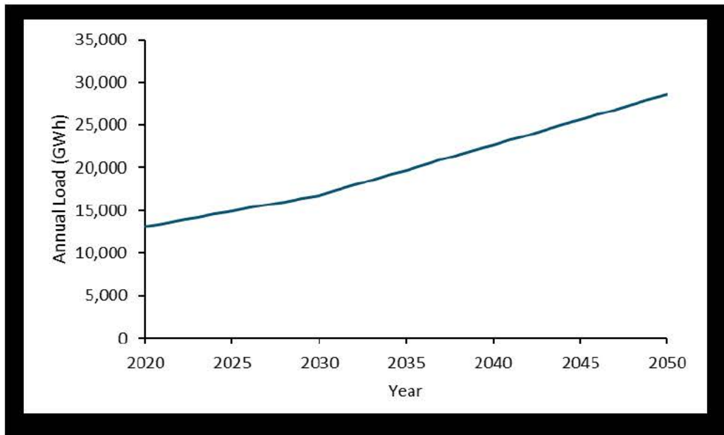
Figure 7. Load forecast used in this study
