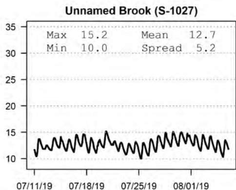
Figure 3.1.1a 2019 In-Stream Continuous Temperature Data (continued)
