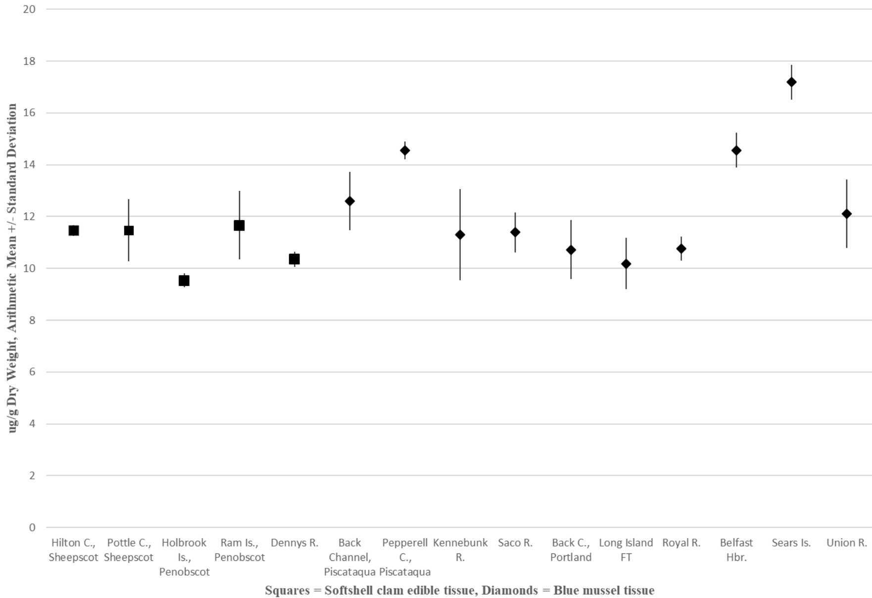
Figure 1.3.1.1.2.1: Arsenic in 2019-20 SWAT Softshell Clam and Blue Mussel Tissue
