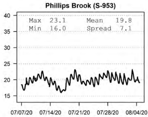
Figure 3.1.1b 2020 In-Stream Continuous Temperature Data (continued)
