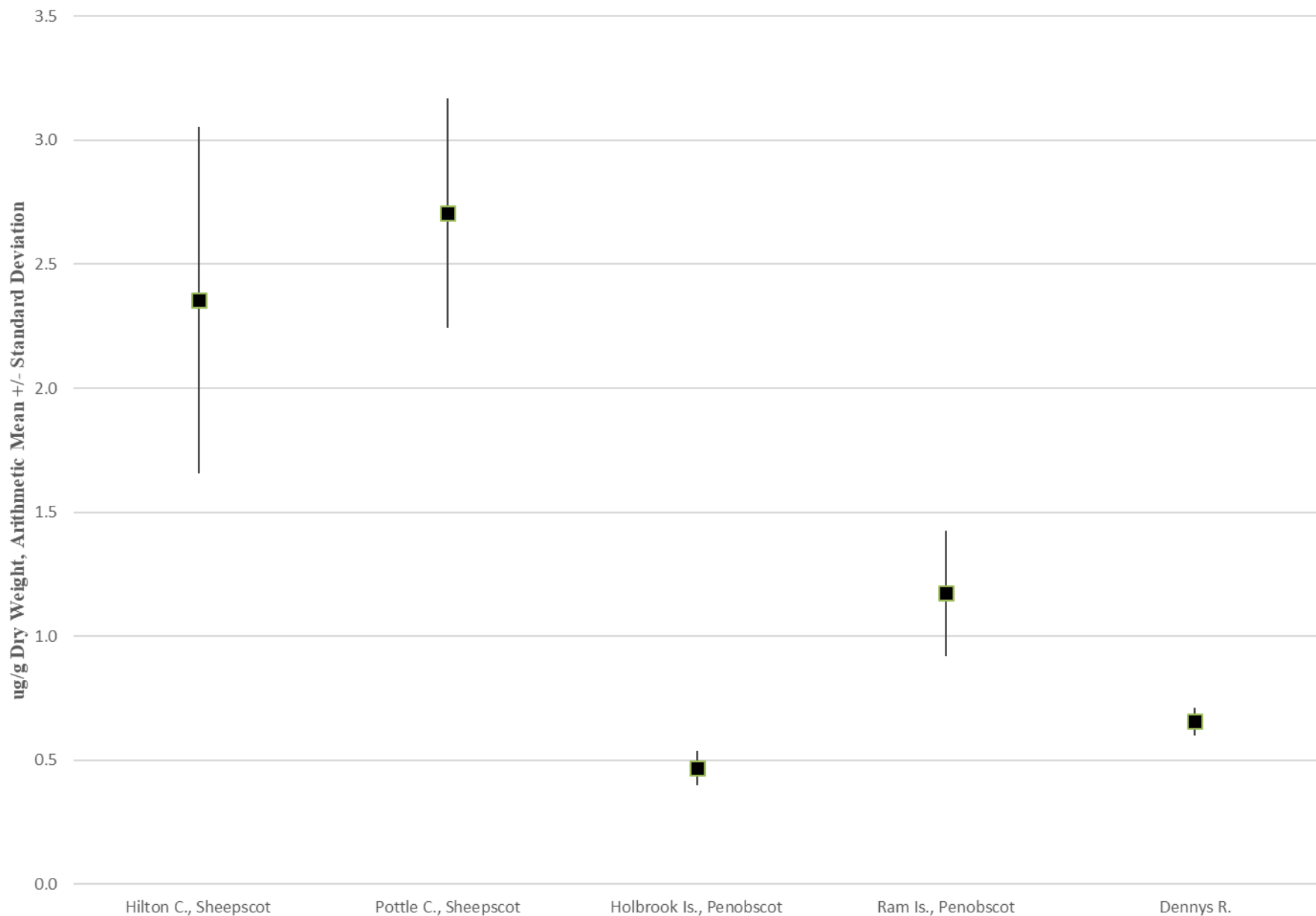
Figure 1.3.1.1.1.1: Silver in 2019 SWAT Softshell Clam Edible Tissue
