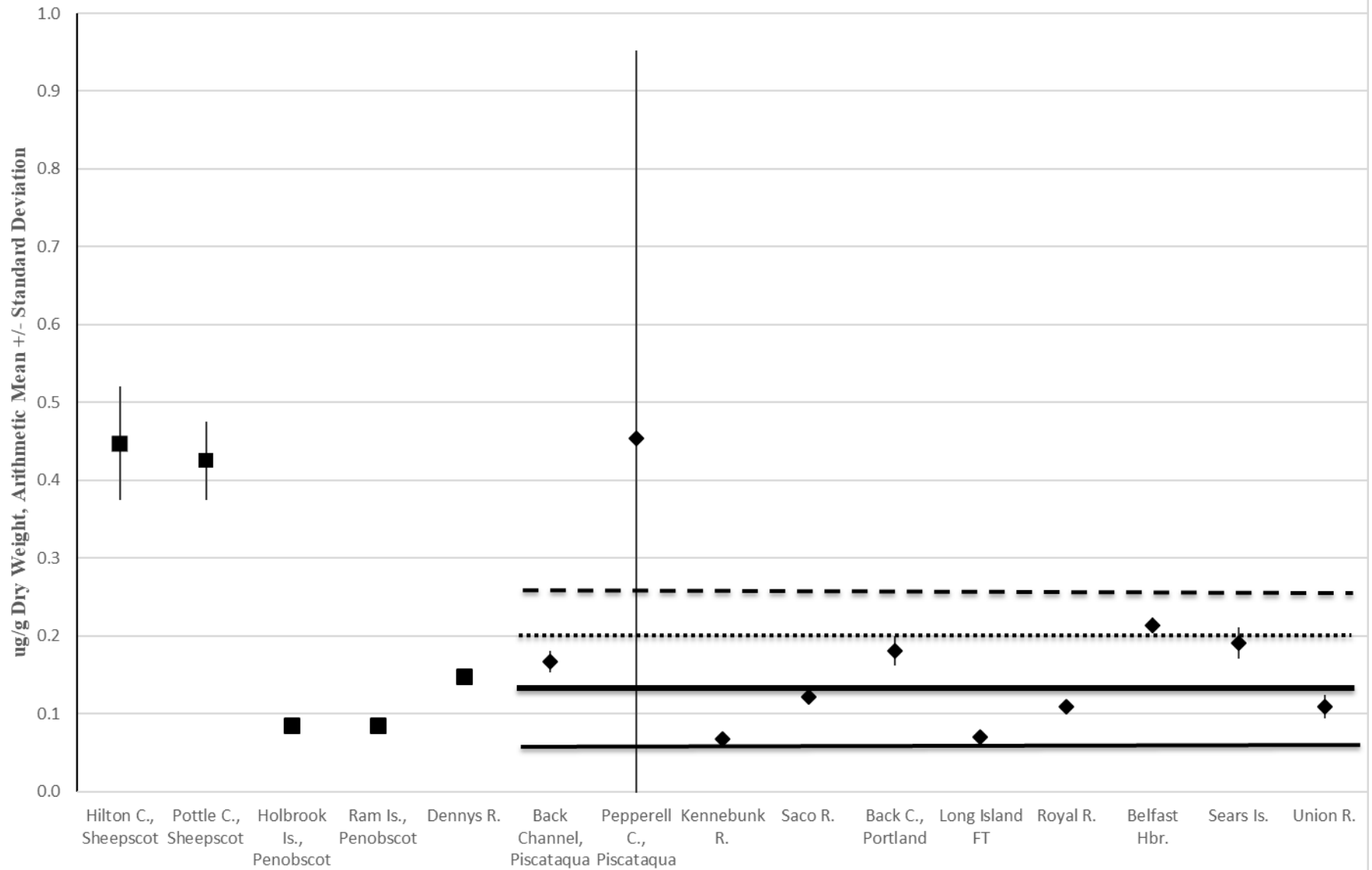
Figure 1.3.1.1.9.1: Mercury in 2019-20 SWAT Softshell Clam and Blue Mussel Tissue
