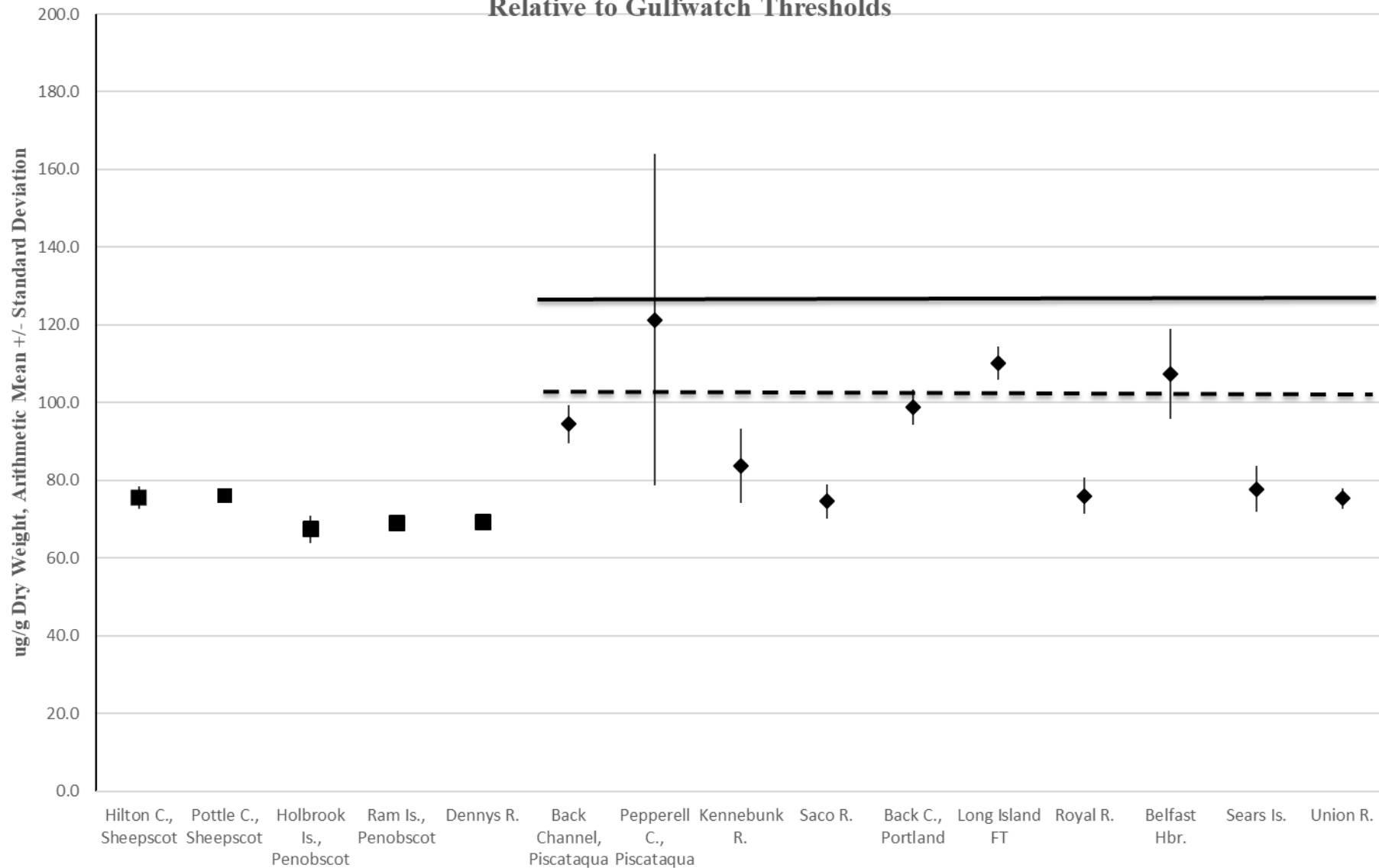
Figure 1.3.1.1.10.1: Zinc in 2019-20 SWAT Softshell Clam and Blue Mussel Tissue Relative to Gulfwatch Thresholds
