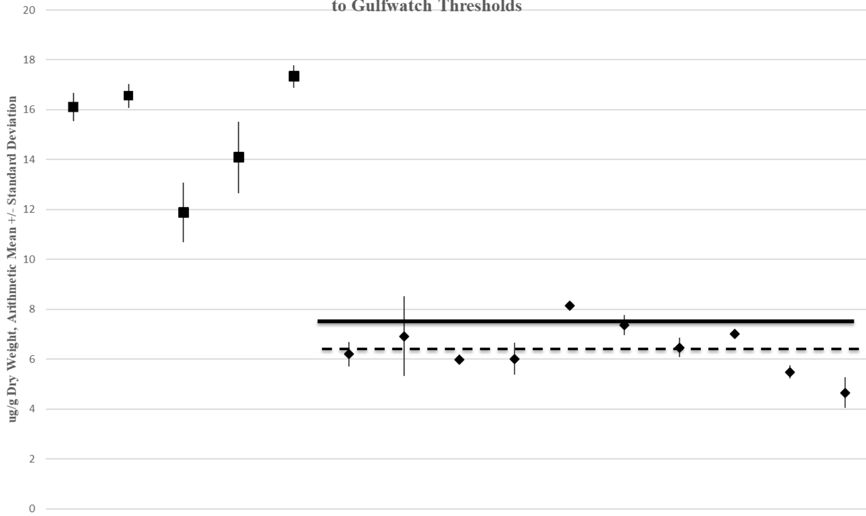
Figure 1.3.1.1.5.1: Copper 2019-20 Softshell Clam and Blue Mussel Tissue Relative to Gulfwatch Thresholds
