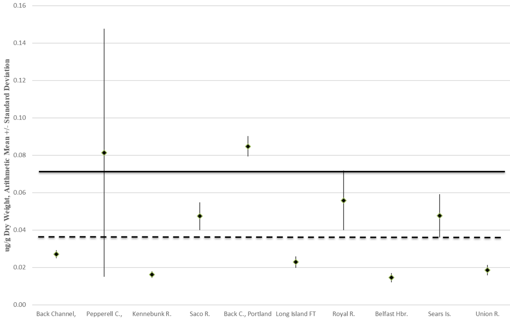
Figure 1.3.1.1.2: Silver in 2020 SWAT Blue Mussel Tissue Relative to Gulfwatch Thresholds
