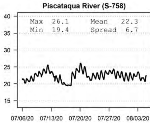
Figure 3.1.1b 2020 In-Stream Continuous Temperature Data (continued)
