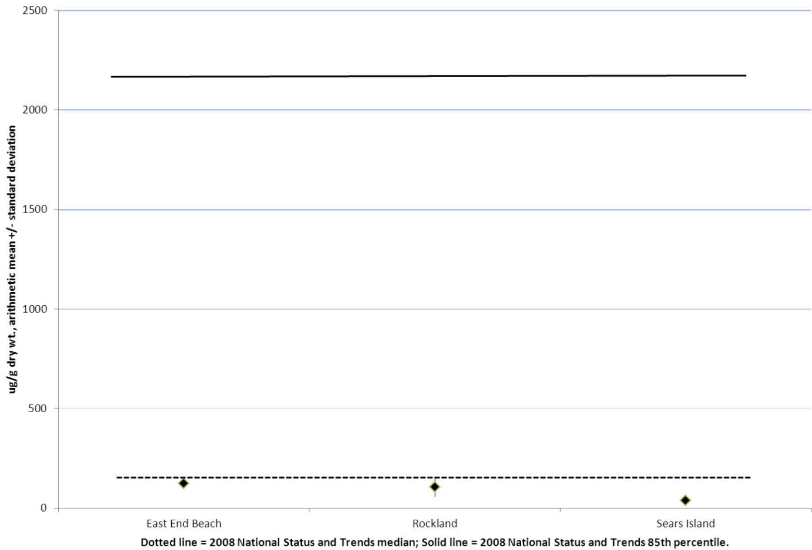
Figure 1.3.1.1.10.2: Zinc in 2013 SWAT Blue Mussels
