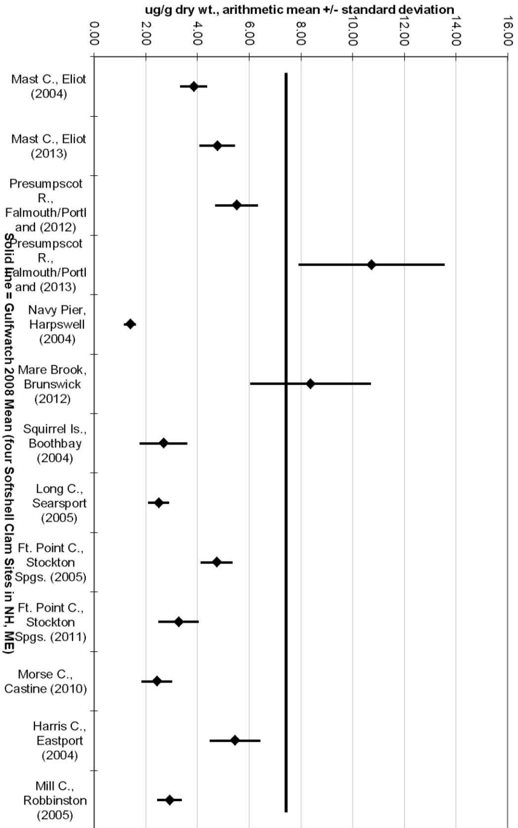
Figure 1.3.1.2.8.1: Lead in SWAT Softshell Clams
