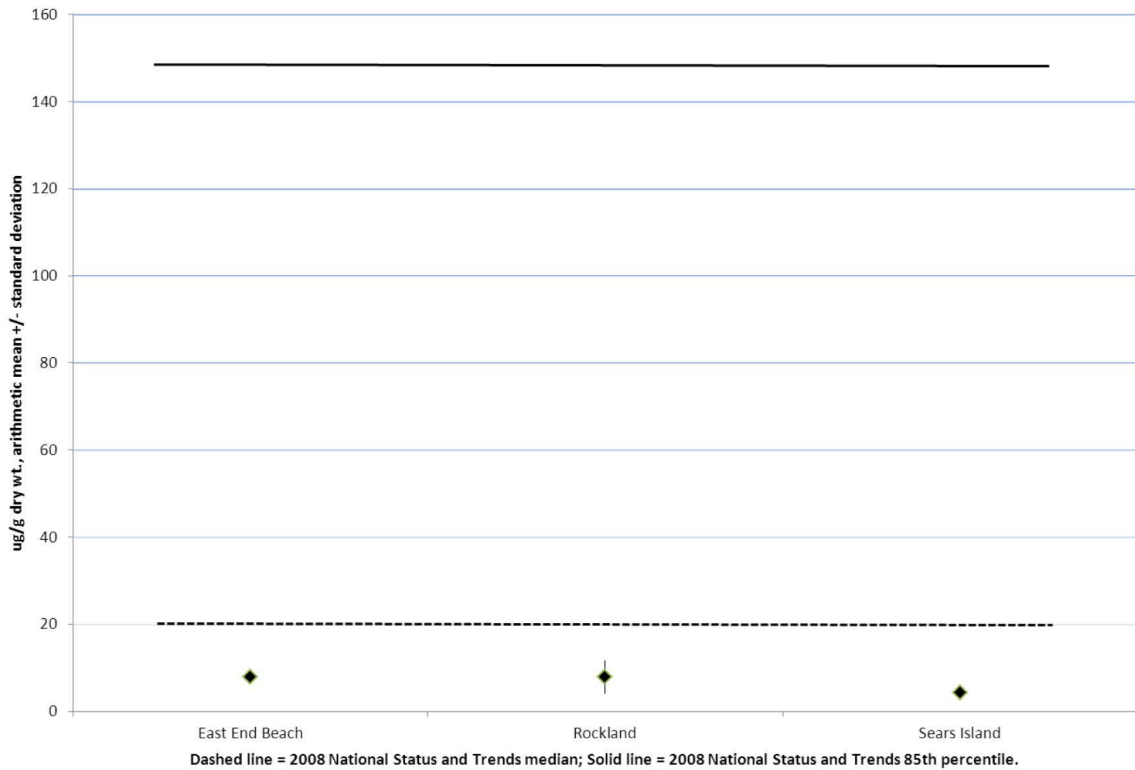
Figure 1.3.1.1.5.2: Copper in 2013 SWAT Blue Mussels
