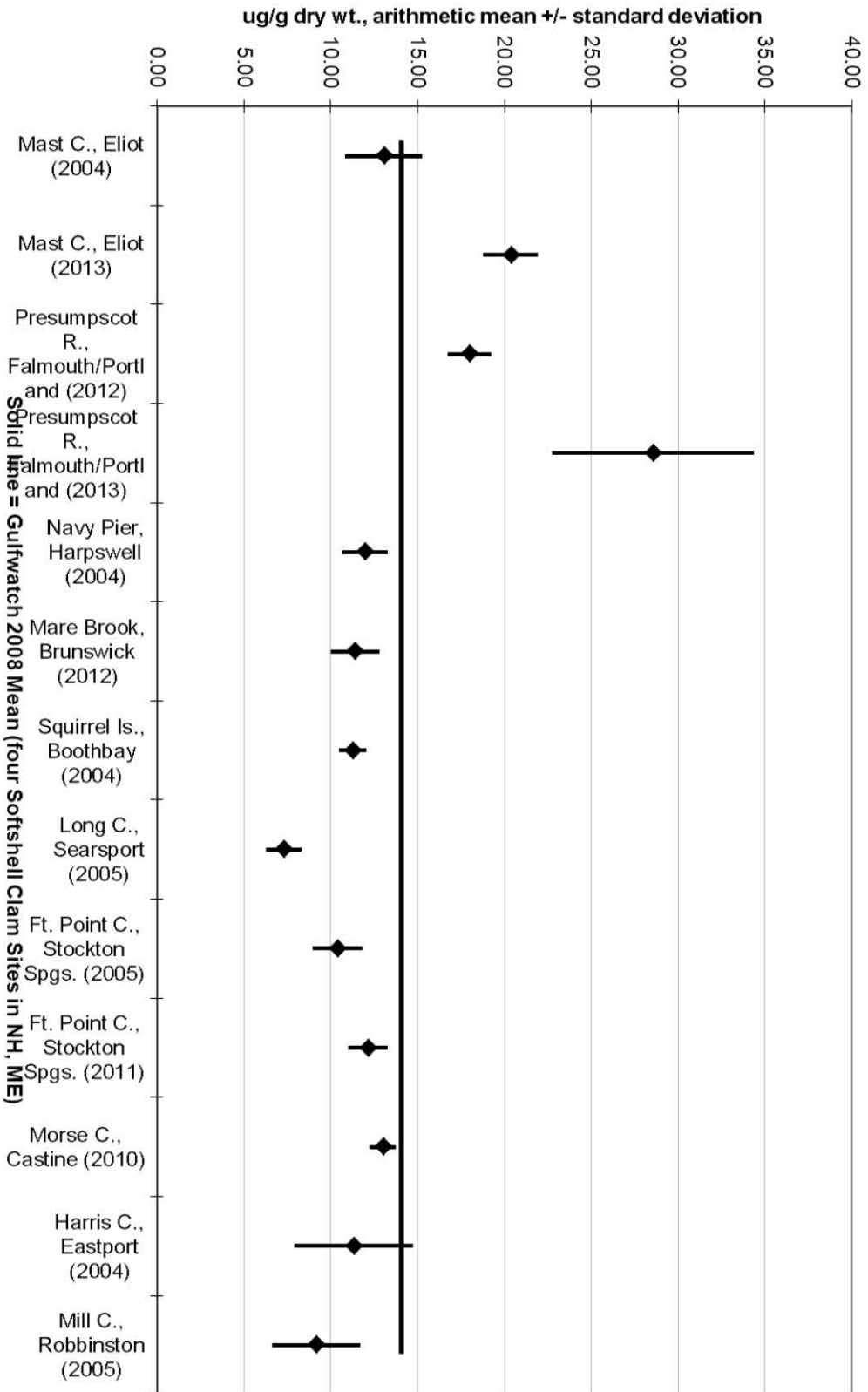
Figure 1.3.1.2.5.1: Copper in SWAT Softshell Clams
