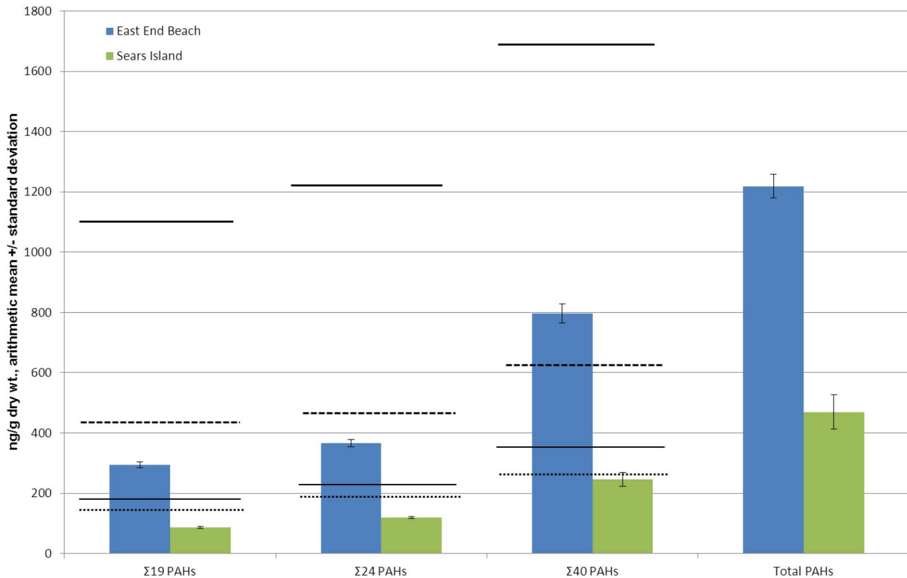
Figure 1.3.2.1.1: PAHs in Blue Mussels
