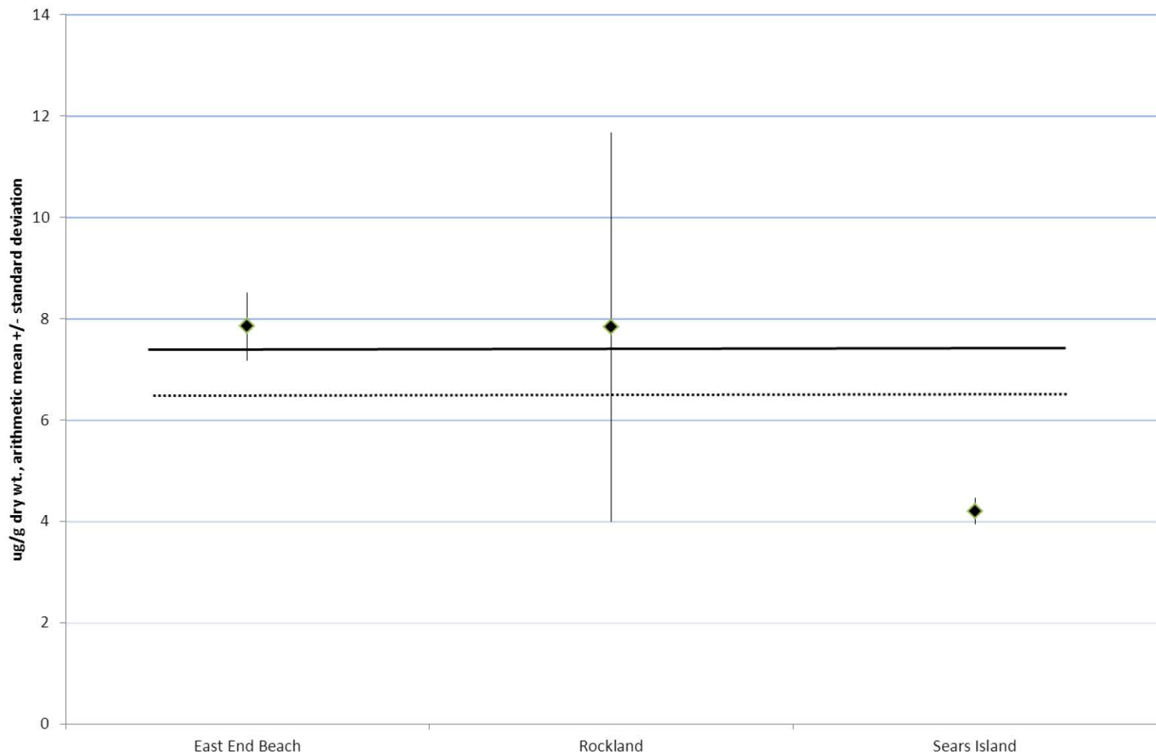
Figure 1.3.1.1.5.1: Copper in 2013 SWAT Blue Mussels
