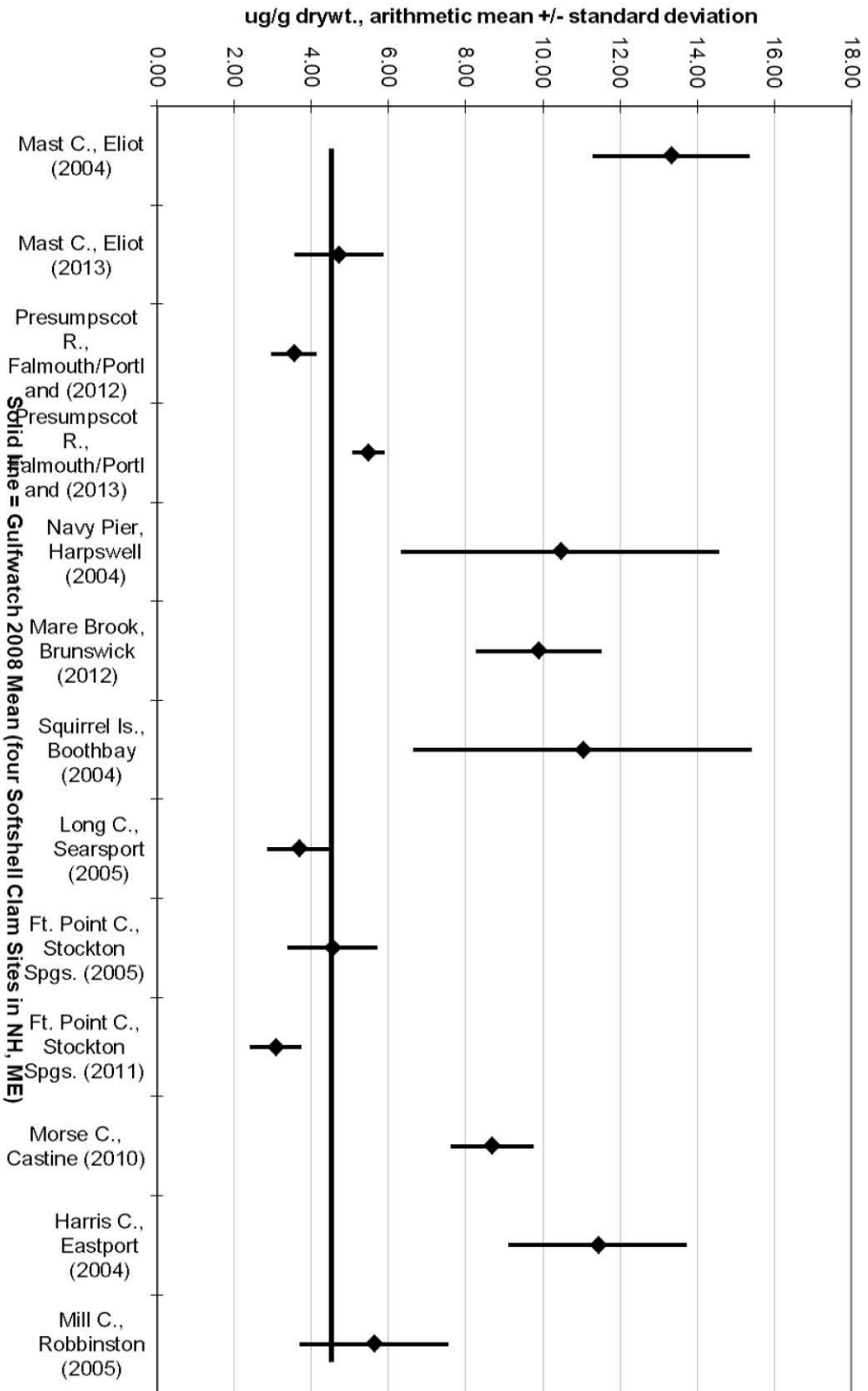
Figure 1.3.1.2.4.1: Chromium in SWAT Softshell Clams
