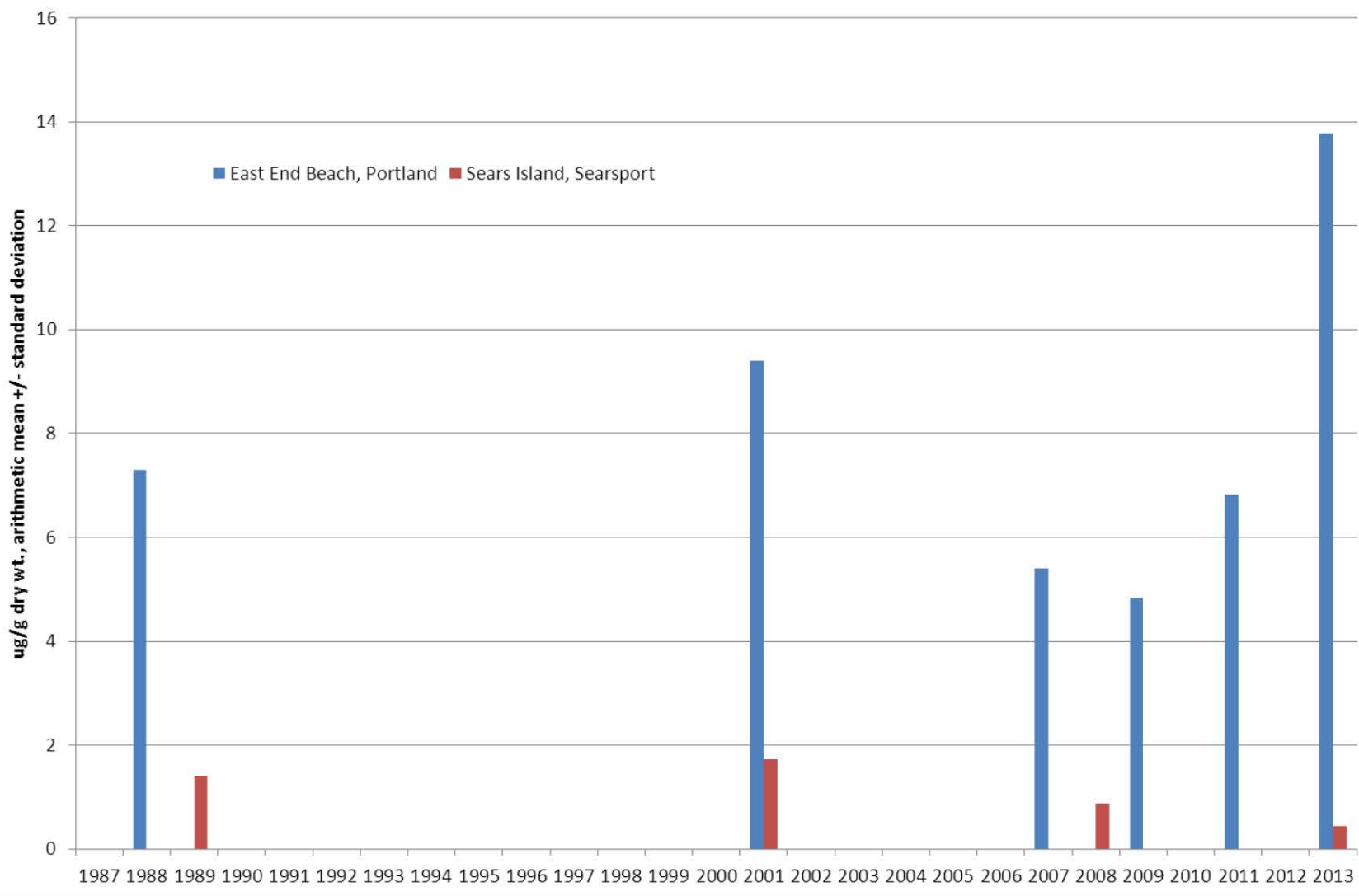
Figure 1.3.1.1.8.2: Trend in Blue Mussel Tissue Lead Concentrations Through 2013
