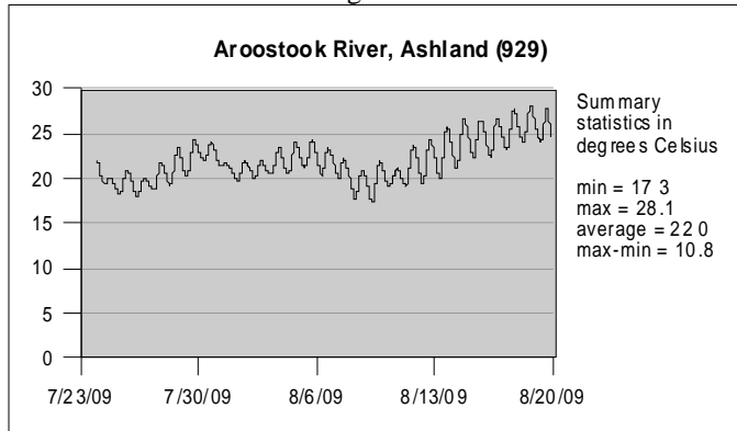
Figure 3.1.1 – 2009 In-Stream Temperature Data Please note: all data are in degrees Celsius
