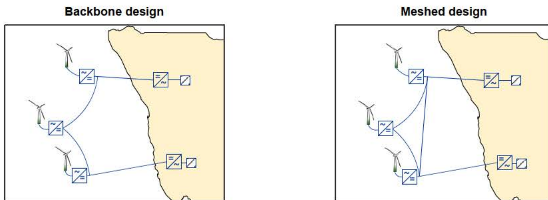
Figure 4-3. Offshore grid with offshore platform interlink*
