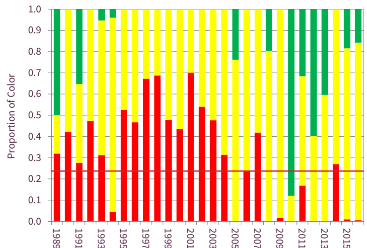
Traffic Light Analysis of Spot (Abundance Metric)
