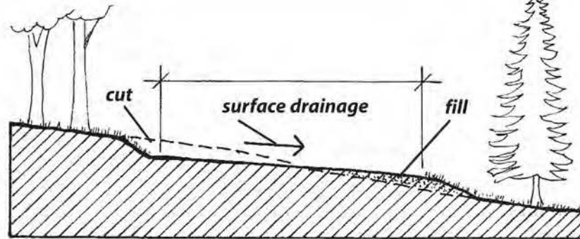
IN-SLOPED ROAD
