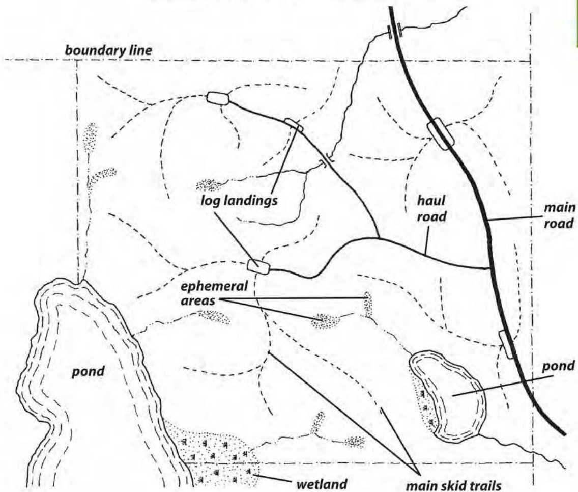
Example of large lot layout.
