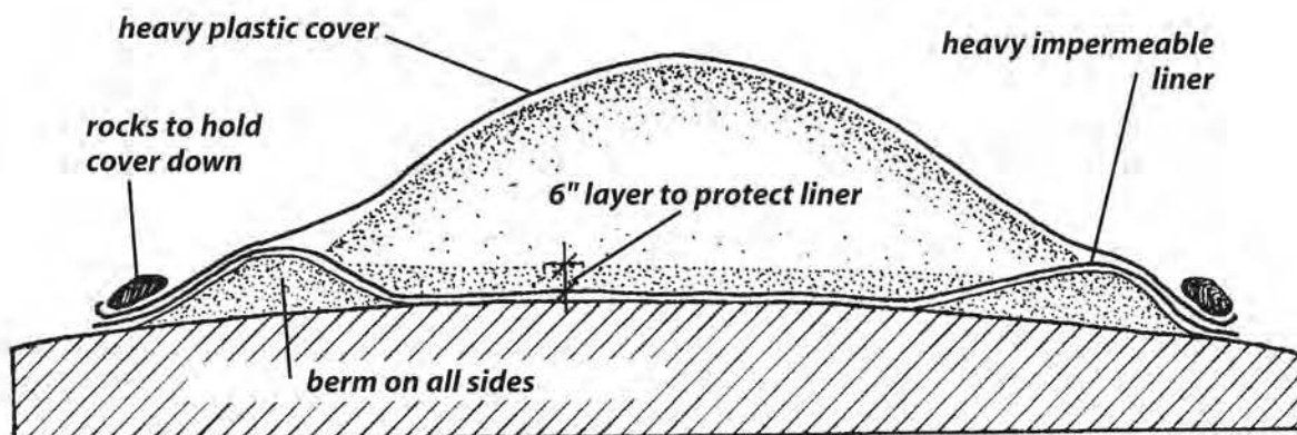
Temporary salt and sand storage pile
