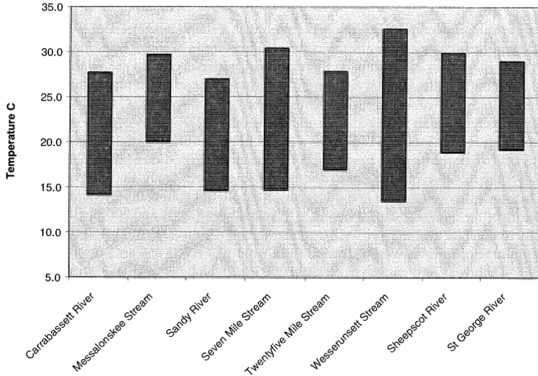
Figure 2. August 2001 maximum and minimum temperatures for main-stem portions of selected southern Maine rivers.
