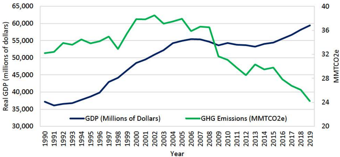
Figure 13. Total GHG emissions and real gross domestic product (GDP)
