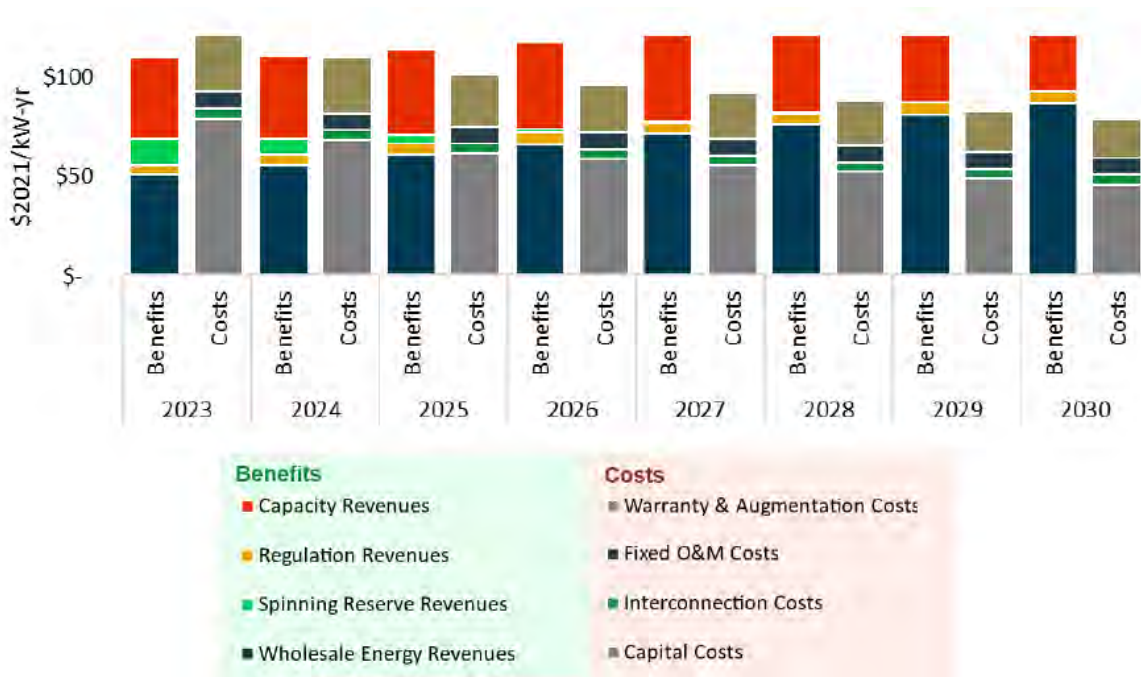
Figure 3: Wholesale standalone storage leveled benefits and costs from participant perspective by storage installation year. [Source: Maine Energy Storage Market Assessment]
