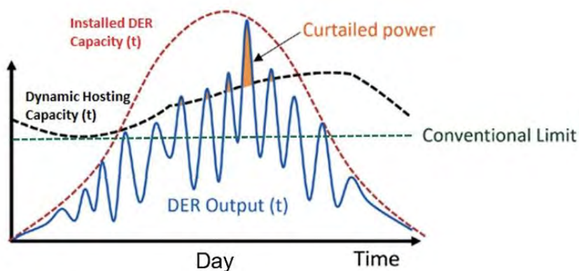
Figure 3 Flexible Interconnection 56
