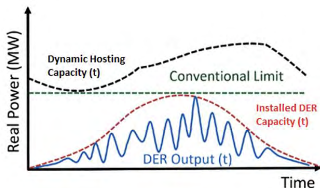
Figure 2 Conventional Interconnection 54
