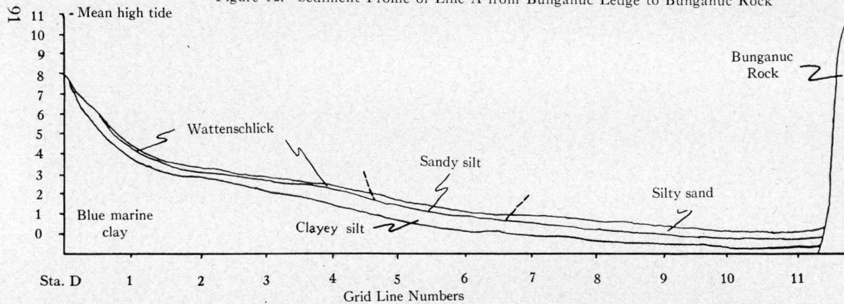
Figure 12. Sediment Profile of Line A from Bunganuc Ledge to Bunganuc Rock
