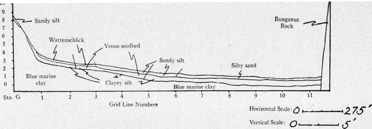
Figure 14. Sediment Profile of Line G from Bunganuc Shore to Bunganuc Rock
