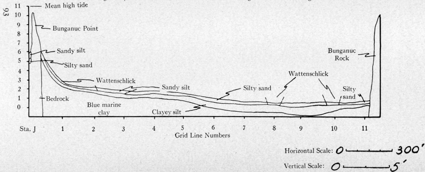
Figure 15. Sediment Profile of Line J from Bunganuc Point to Bunganuc Rock
