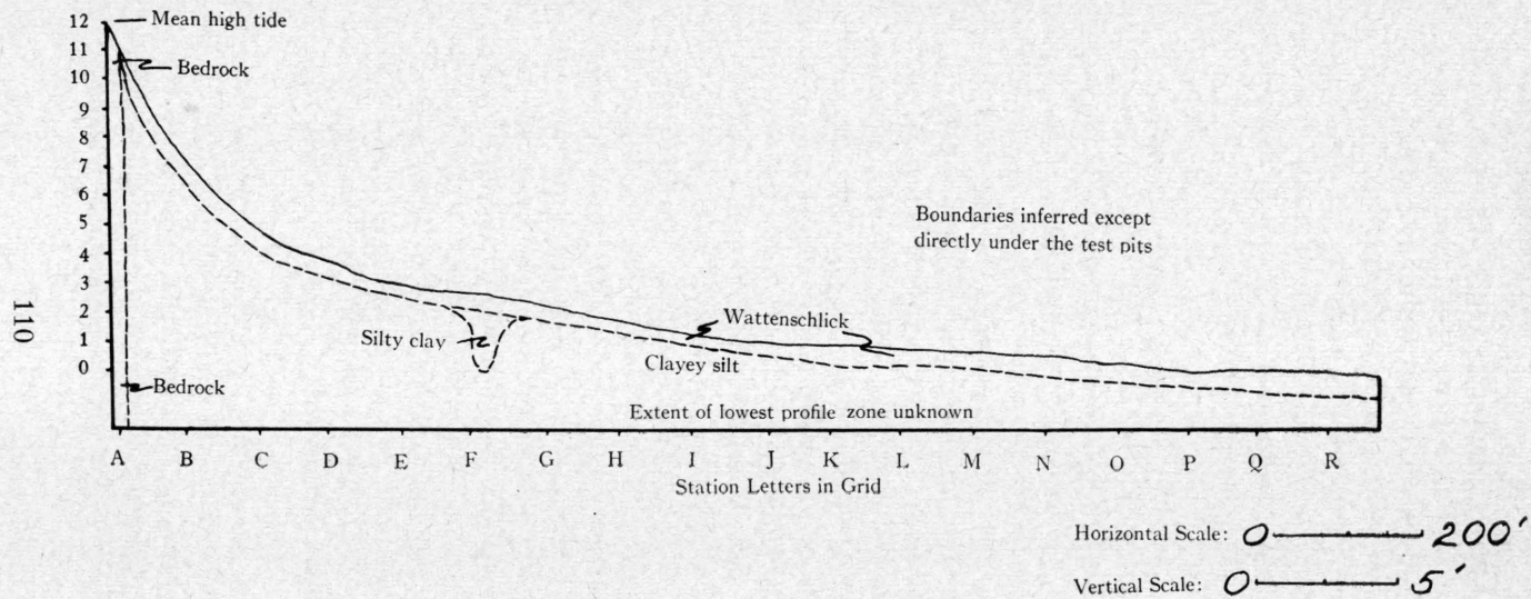
Figure 24. Sediment Profile along Grid Line Number 6 from Grid Letter A to Grid Letter R
