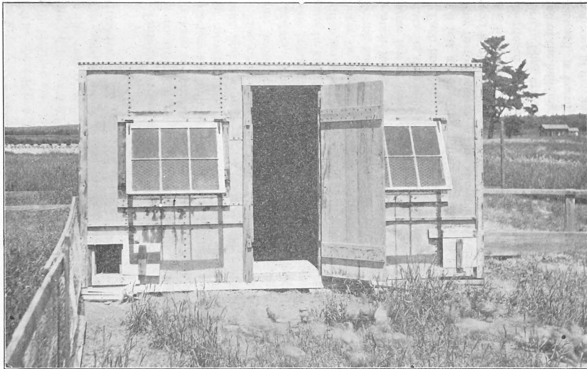
Figure 10. Movable brooder house. Described on page 52.
