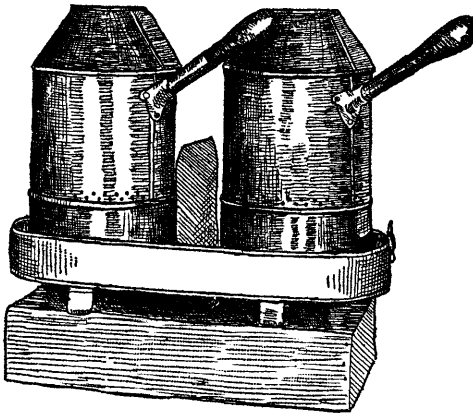
Bowdoin Generator—Double.
