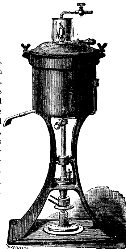
COMPLETE VIEW.
