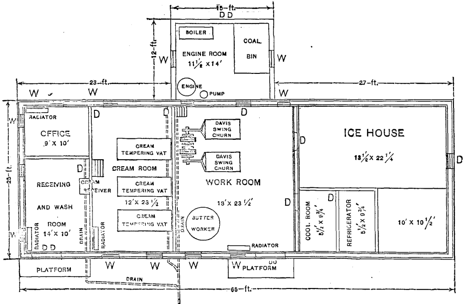
LEMONT CREAMERY—FLOOR PLAN.
