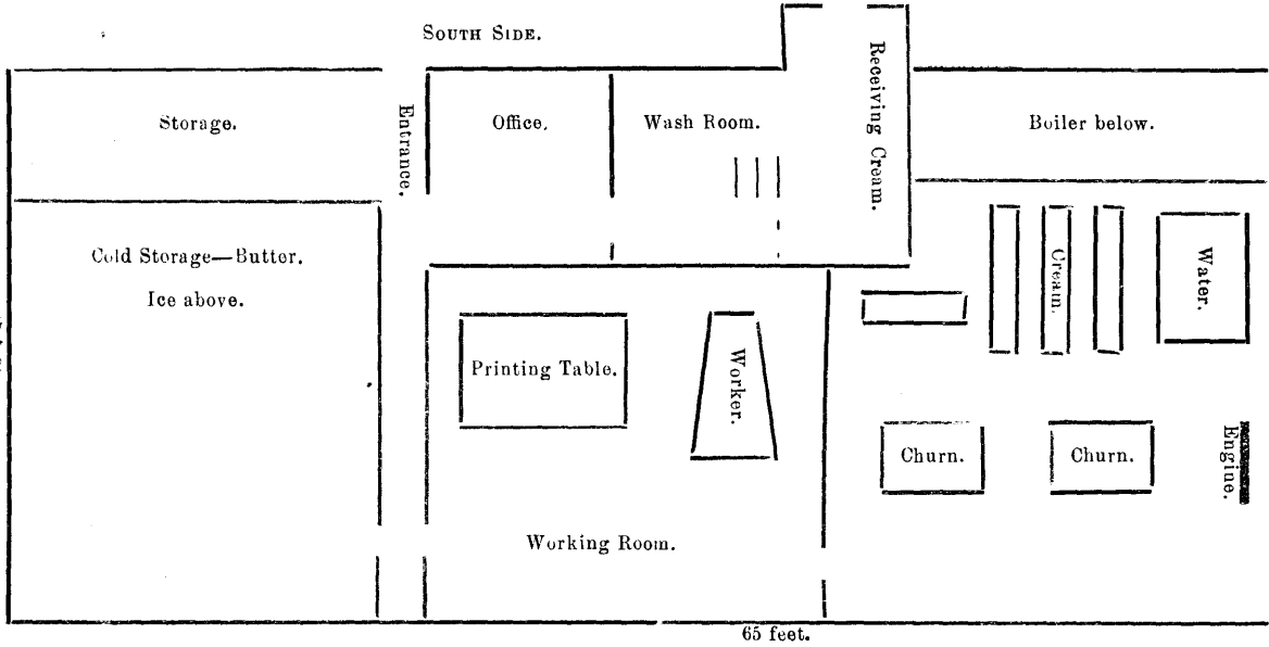
PLAN OF TURNER CENTER CREAMERY.
