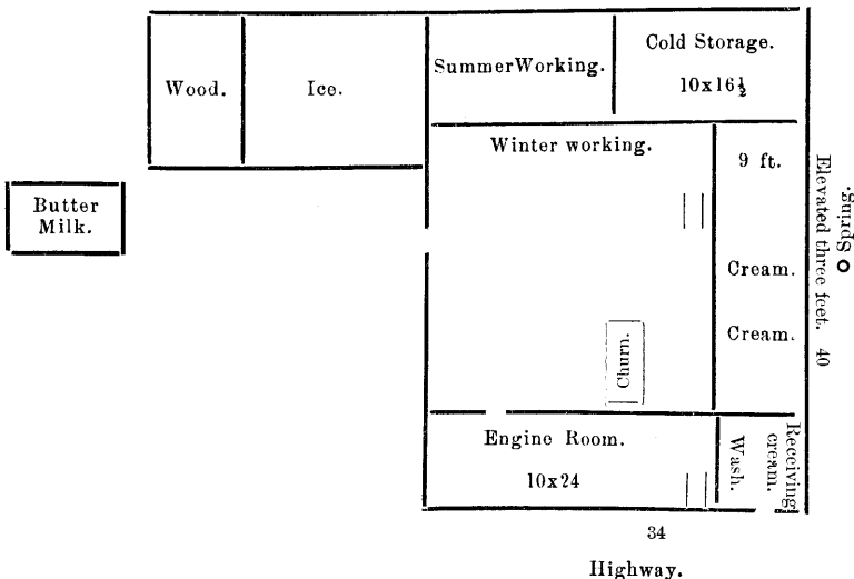
PLAN OF BUCKFIELD CREAMERY.
