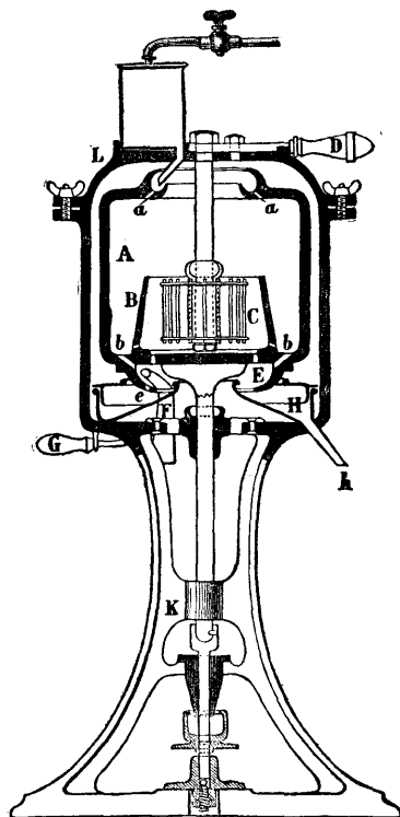
SECTIONAL VIEW.
