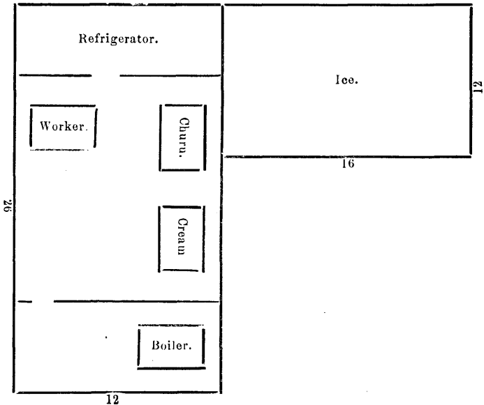
PLAN OF SMALL CREAMERY.
